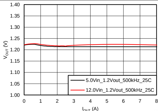
Figure 23. Load Regulation Performance
