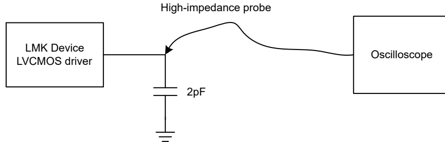
Figure 7-3. LVCMOS Output Time Domain Test Configuration
