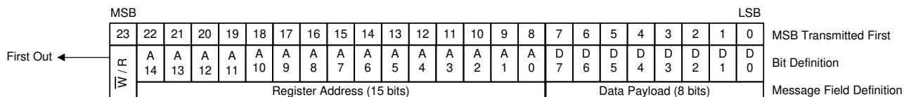
Figure 8-44. SPI Message Format
