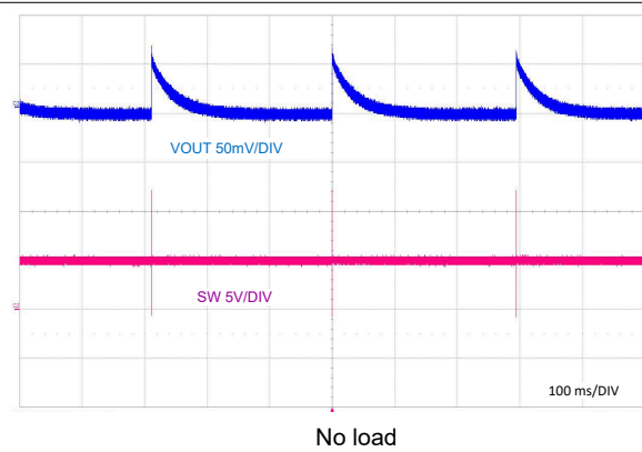
Figure 9-22. PFM Switching
