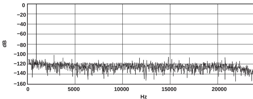
Figure 10. DAC FFT Plot ( T_A = 25^\circ\text{C} , 48\text{ kpsps} , 0\text{ dB} , 1\text{ kHz} Input, \text{AVDD} = 3.3\text{ V} , R_L = 10\text{ k}\Omega )
