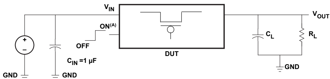
Figure 29. Test Circuit
