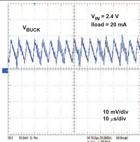
Figure 5. Buck Output-Voltage Ripple, PFM
