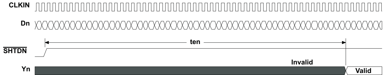
Figure 10. Enable Time Waveforms
