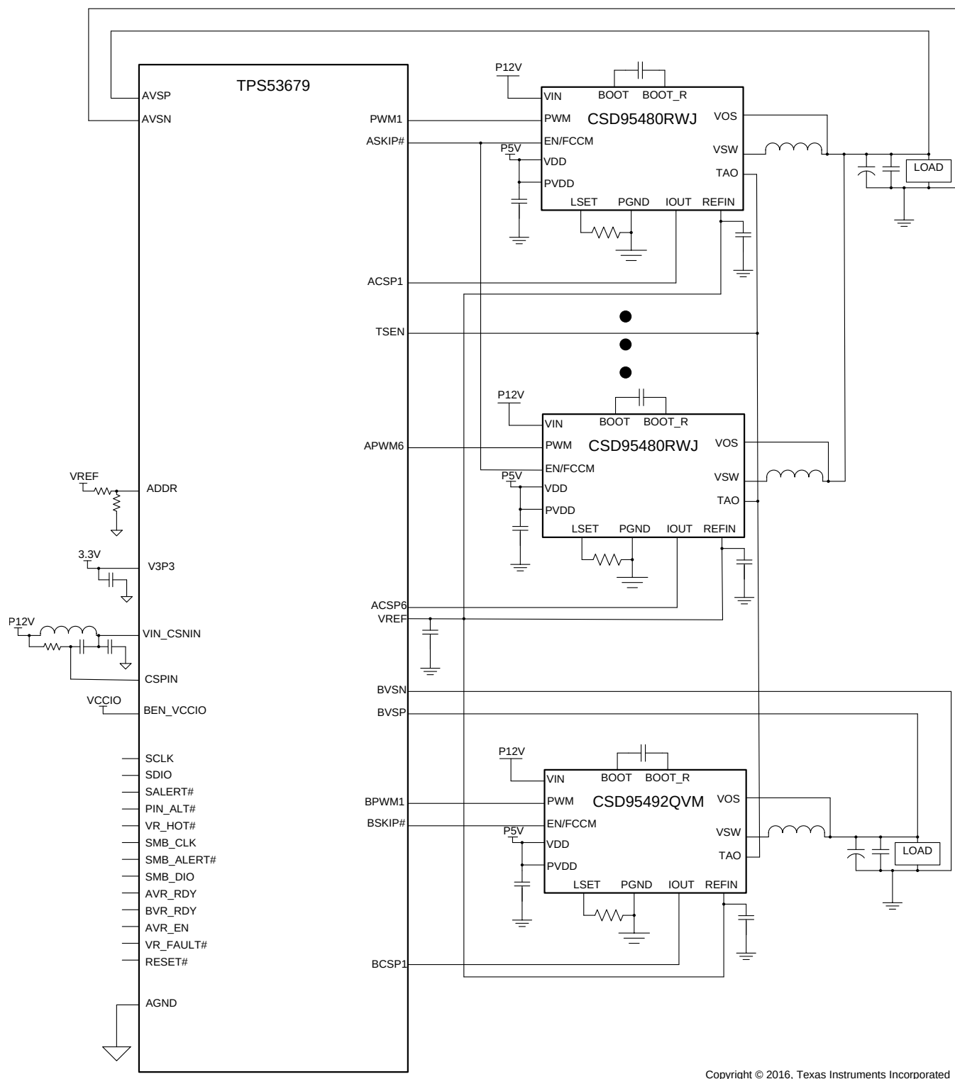
Figure 1. Application Schematic
