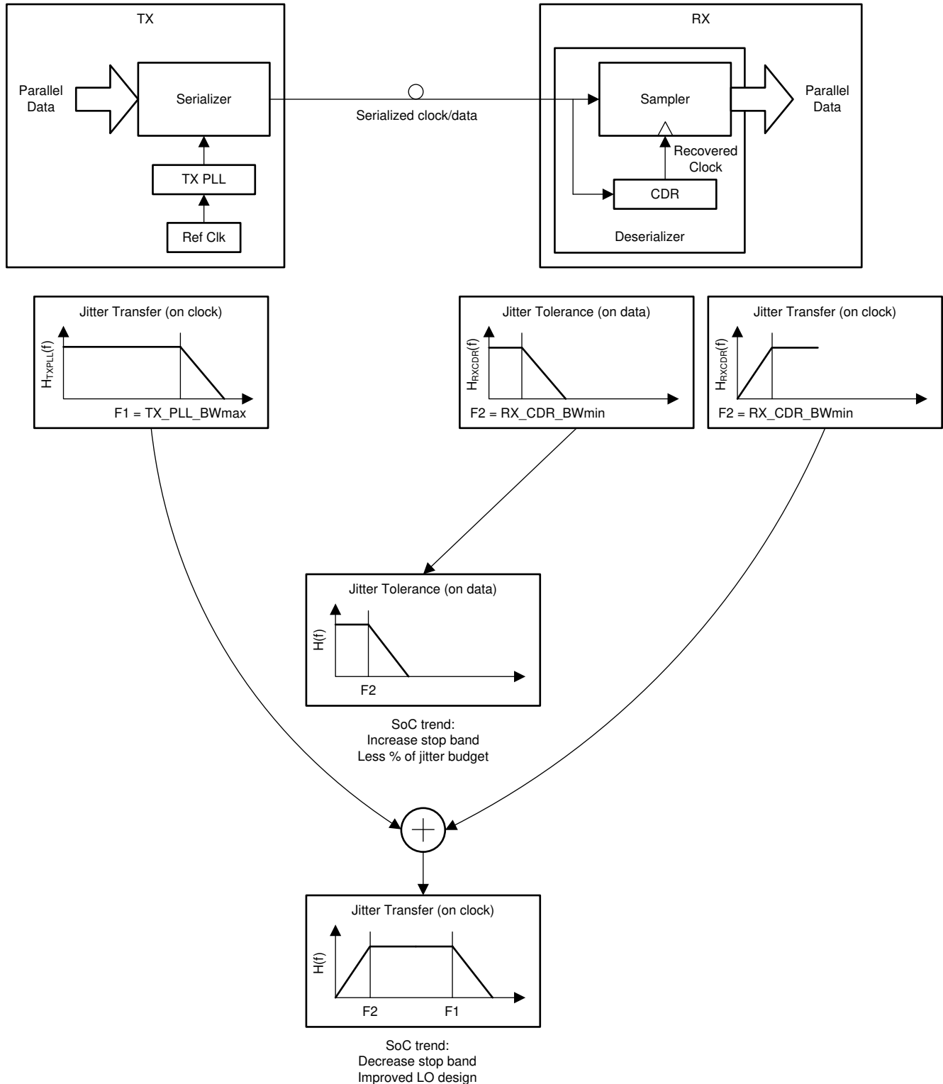
Figure 10-1. Dependence of Clock Jitter in Serial Links
