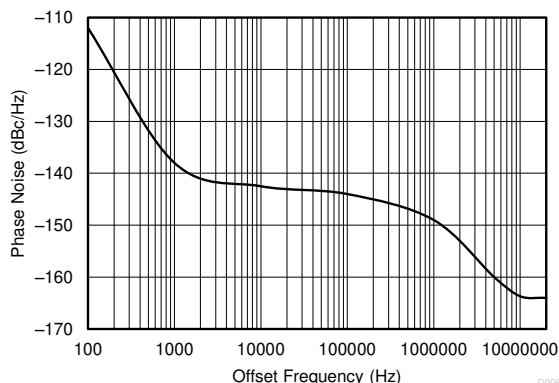
Figure 6-3. Closed-Loop Phase Noise of AC-LVDS Outputs at 156.25 MHz With PLL Bandwidth at 1 MHz, Integer N PLL, 50-MHz Crystal Input, 5-GHz VCO Frequency, Post Divider = 8, Output Divider = 4
