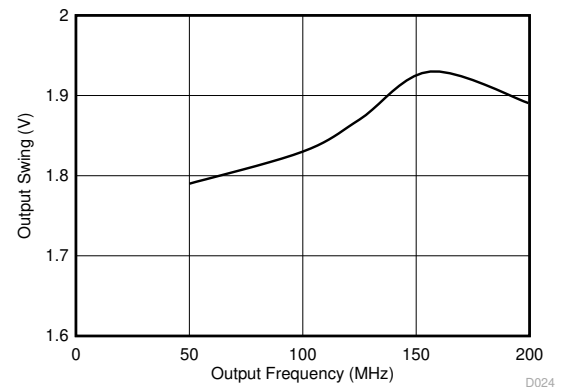
Figure 6-22. 1.8-V LVCMOS (on OUT[7:0]) Output Swing vs. Frequency
