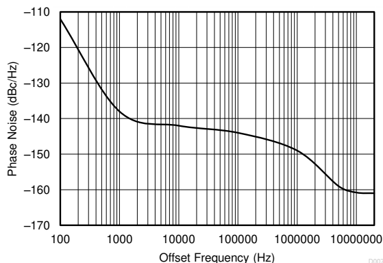
Figure 6-5. Closed-Loop Phase Noise of HCSL Outputs at 156.25 MHz With PLL Bandwidth at 1 MHz, Integer N PLL, 50-MHz Crystal Input, 5-GHz VCO Frequency, Post Divider = 8, Output Divider = 4
