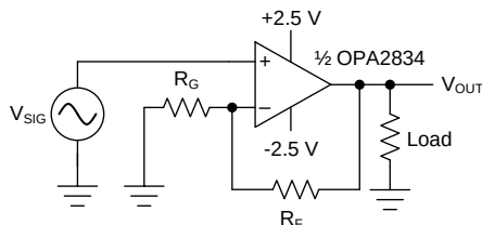
Figure 50. Split-Supply Operation
