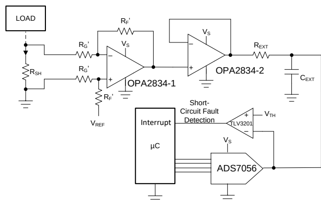
Low-Side, Current-Shunt Monitoring
