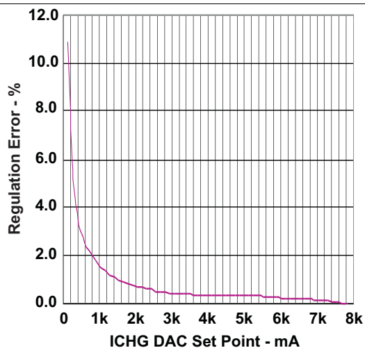
Figure 6. Charge Current Regulation Accuracy vs V(CSOP-CSN) Voltage Set Point
