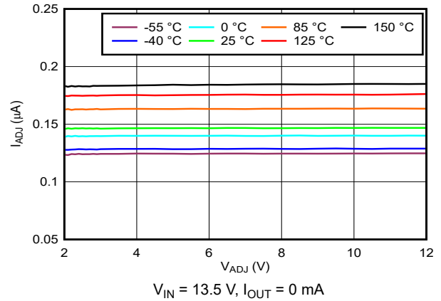
Figure 6-14. Adjustable Pin Current vs. Adjustable Pin Voltage
