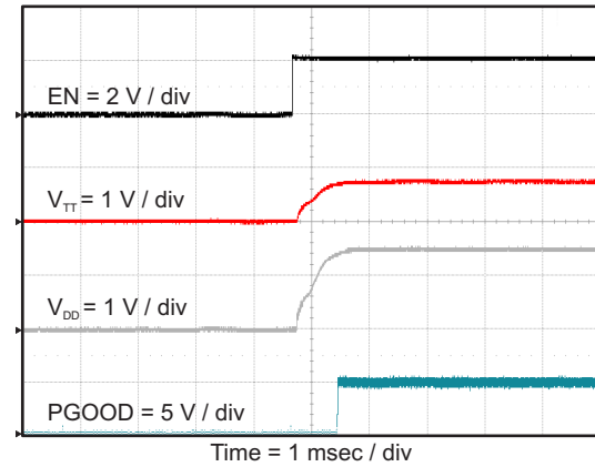
Figure 54. V TT and V DD Start-Up Relative to Enable
