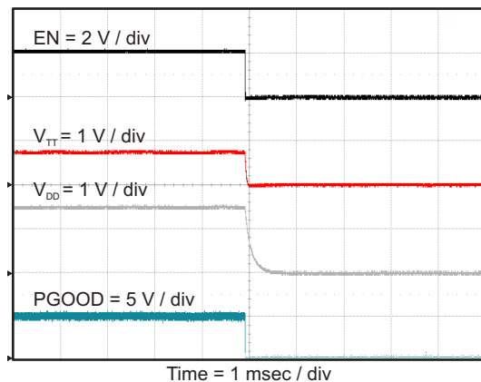
Figure 57. V TT and V DD Shutdown Relative to Enable
