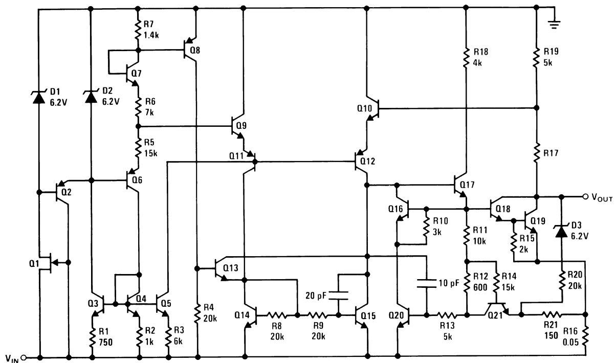
Figure 3. -5V
