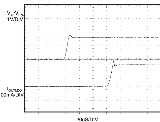
Figure 36. Short-Circuit Response Time (LDO Power Up to Hard Short) (TPS22949)
