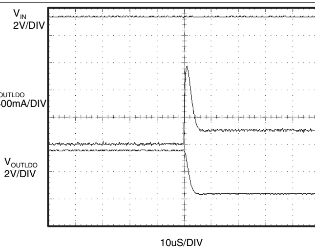
Figure 34. Short-Circuit Response Time ( V_{OUTLDO} Shorted to GND)
