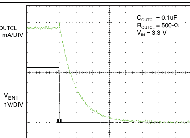
Figure 32. Current Limiter t_{OFF} Response
