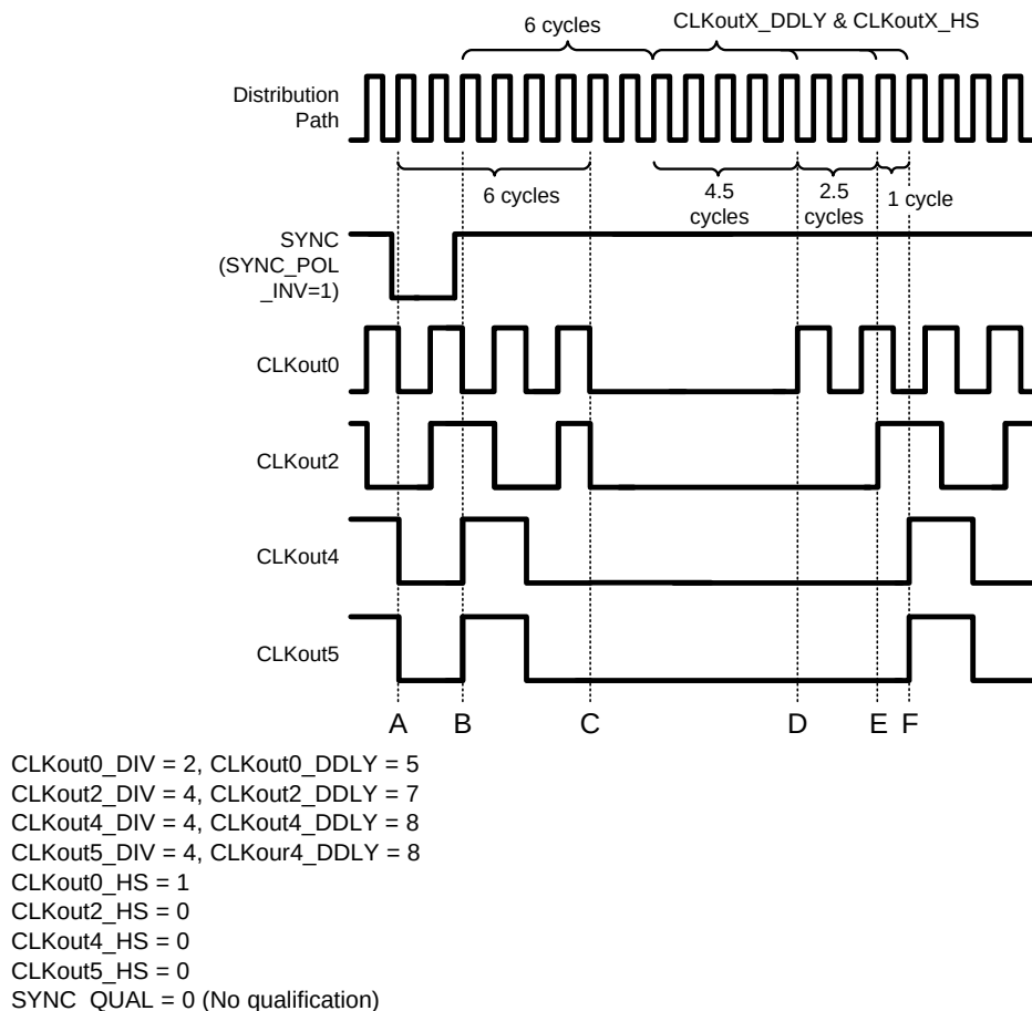
Figure 12. Clock Output Synchronization Using the SYNC Pin (Active Low)
