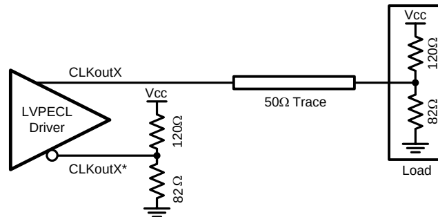
Figure 33. Single-Ended LVPECL Operation, DC Coupling, Thevenin Equivalent
