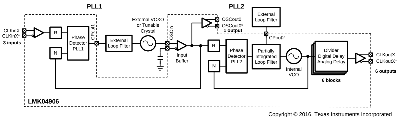
Figure 37. Simplified Functional Block Diagram for Dual Loop Mode
