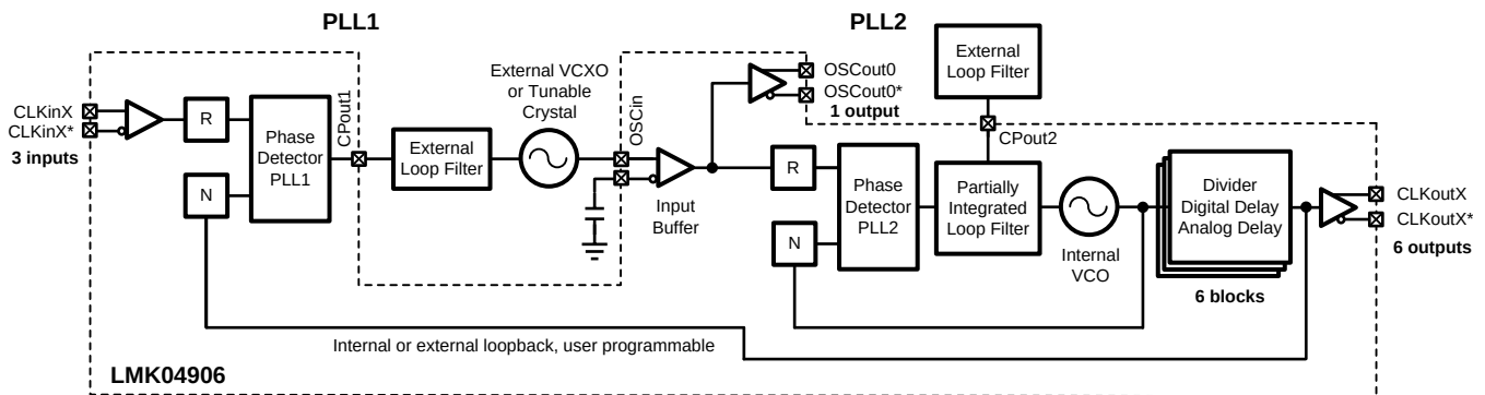
Figure 16. Simplified Functional Block Diagram for 0-delay Dual Loop Mode
