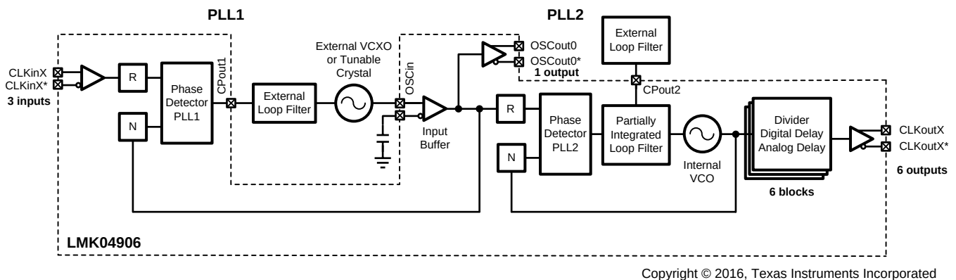
Figure 15. Simplified Functional Block Diagram for Dual Loop Mode
