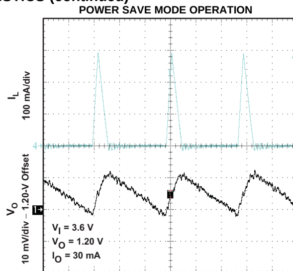
t – Time = 500 ns/div Figure 42.
