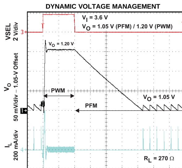
t – Time = 25 \mu\text{s/div} Figure 44.
