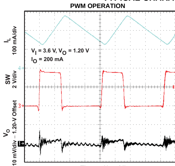
t – Time = 40 ns/div Figure 41.
