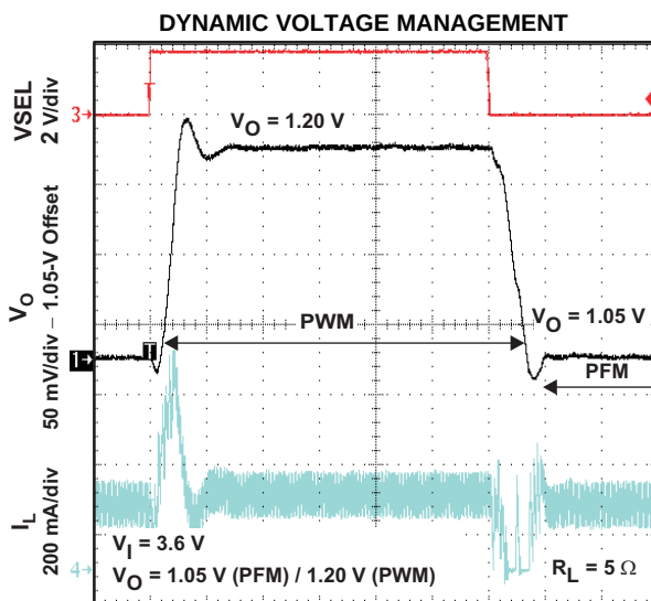
t – Time = 5 \mu\text{s/div} Figure 43.
