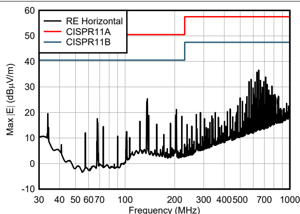
Figure 9-6. AMC131M03 Horizontal Radiated Emission CISPR11 Measurement
