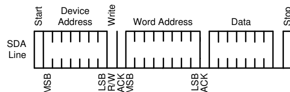
Figure 12. SMBus Write Operation
