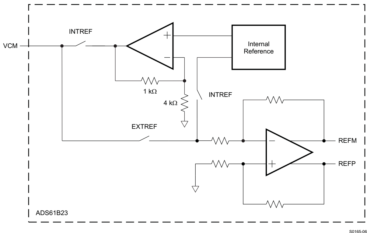
Figure 37. Reference Section
