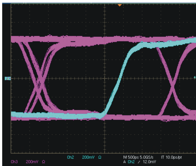
Figure 46. LVDS Eye Diagram with 100-Ω Internal Termination 10-pF Load Capacitance Blue Trace - Output Clock (CLKOUT) Pink Trace - Output Data
