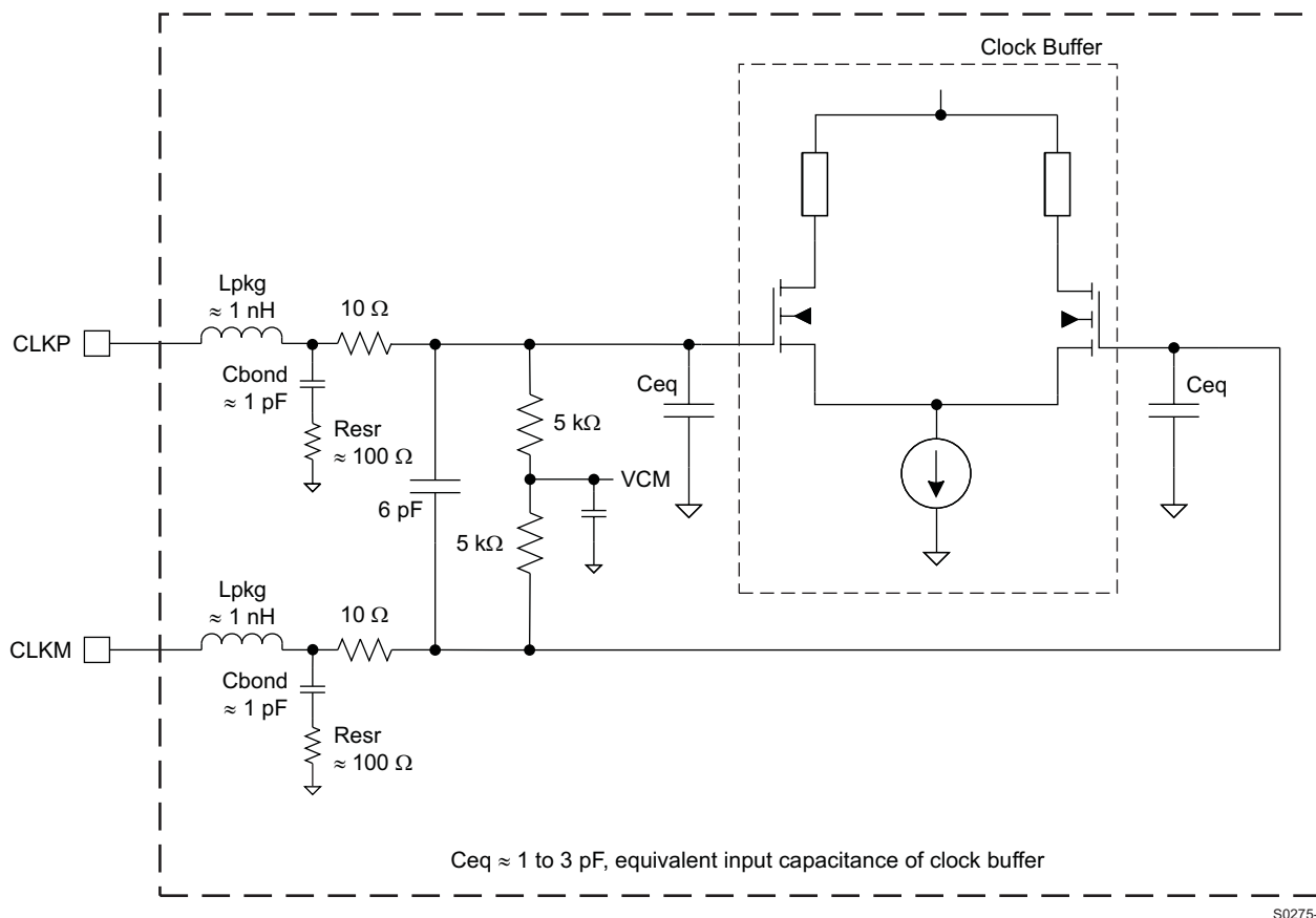
Figure 38. Internal Clock Buffer
