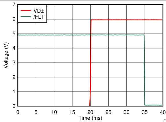
Figure 14. \overline{\text{FLT}} Assertion Time During OVP
