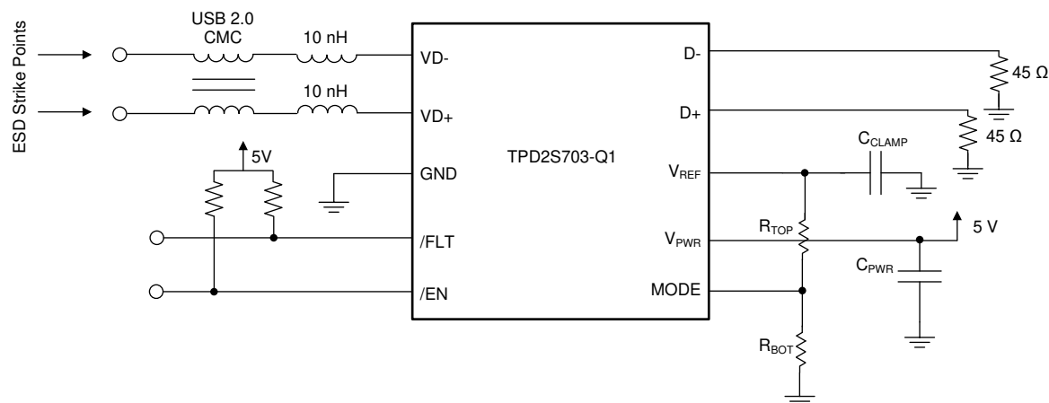
Figure 20. ESD Setup
