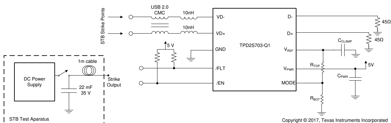
Figure 21. Short-to-Battery Setup
