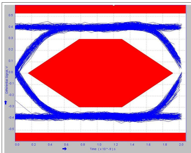
Figure 24. USB2.0 Eye Diagram (Board Only, Through Path)
