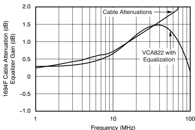
Figure 87. Cable Attenuation versus Equalizer Gain
