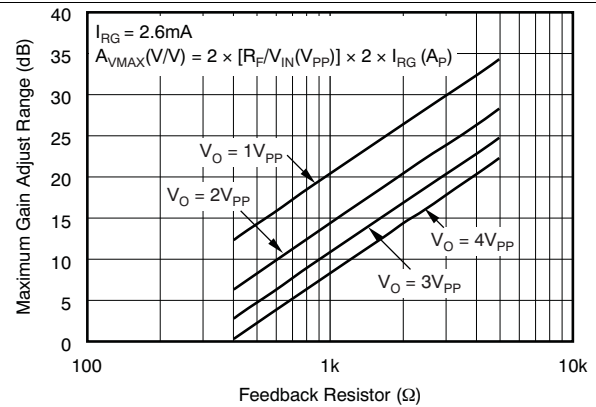
Figure 2. Maximum Gain Adjust Range vs R_F
