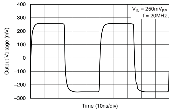
Figure 13. Small-Signal Pulse Response
