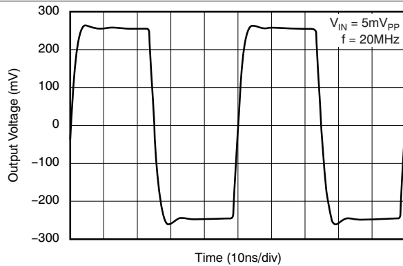
Figure 55. Small-Signal Pulse Response
