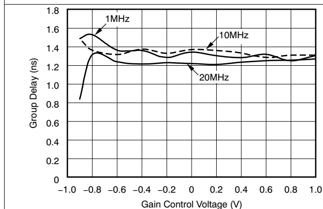
Figure 26. Group Delay vs Gain Control Voltage
