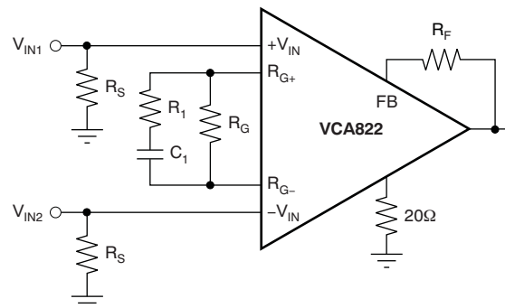
Figure 84. Differential Equalizer
