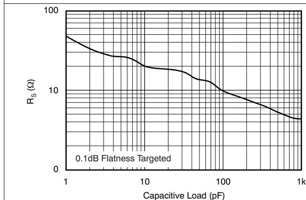
Figure 28. Recommended R_S vs Capacitive Load
