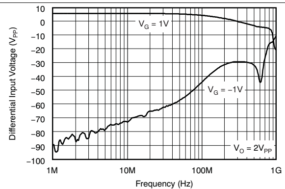
Figure 25. Fully-Attenuated Response
