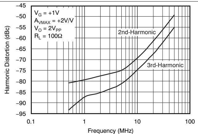
Figure 17. Harmonic Distortion vs Frequency
