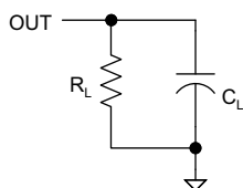
Figure 6-1. Output Rise-Fall Test Load
