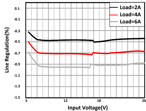
Figure 11-6. Line Regulation
