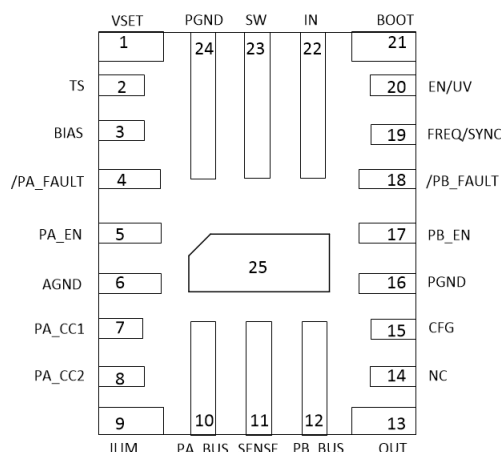
Figure 7-2. TPS25869 RPQ Package 25-Pin (QFN) Top View
