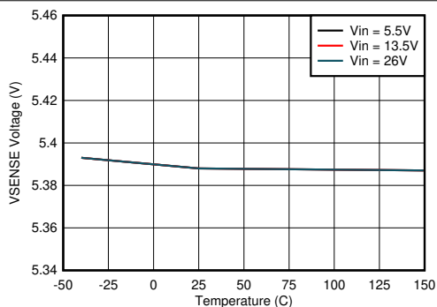
Figure 8-5. V_{\text{SENSE}} Voltage vs Junction Temperature
