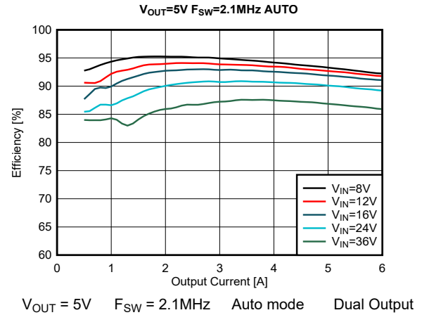
Figure 8-22. Efficiency
