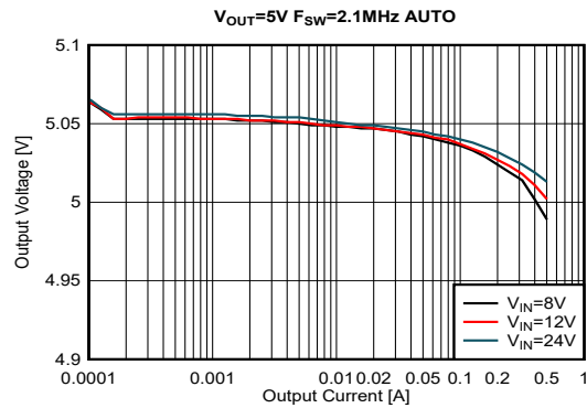
Figure 8-30. Load and Line Regulation
