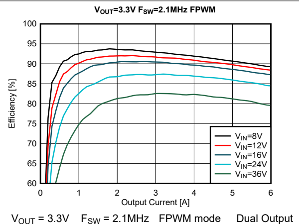
Figure 8-26. Efficiency
