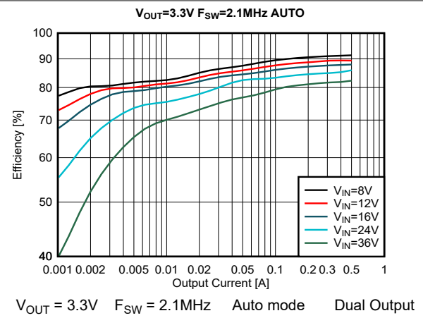
Figure 8-24. Efficiency
