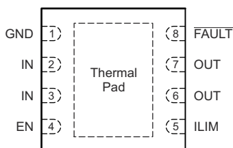
Figure 6-1. 8-Terminal S-PVSON With Thermal Pad DRB Package (Top View)
