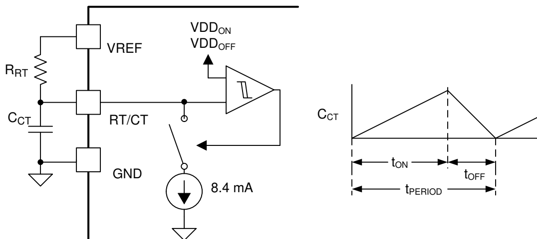
Figure 8-4. Oscillator Circuit
