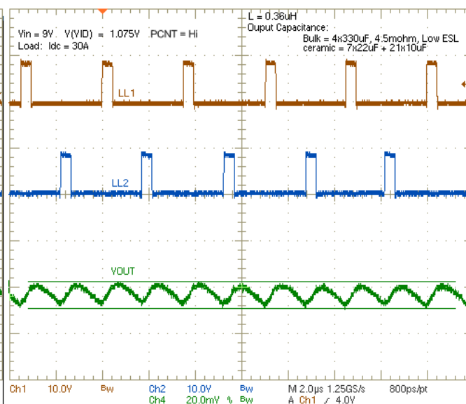
Figure 31. Output Ripple, V_{IN} = 9V
