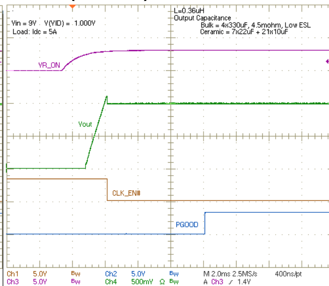
Figure 29. \overline{PG} and PGOOD, V_{IN} = 9V
