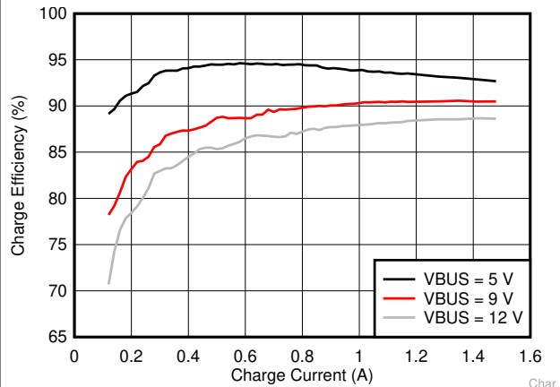
Figure 7-2. Charge Efficiency
