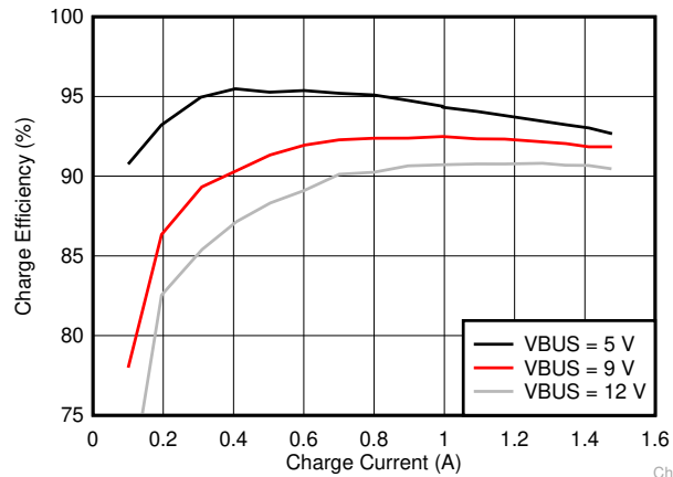
Figure 7-1. Charge Efficiency
