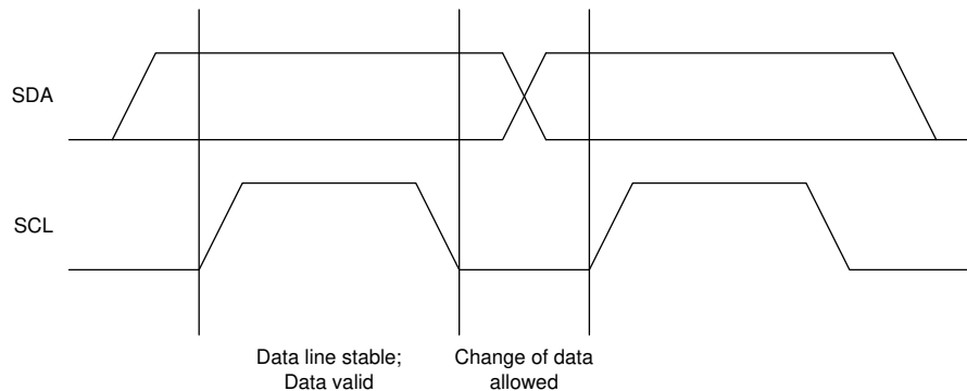
Figure 8-6. Bit Transfer on the I 2 C Bus
