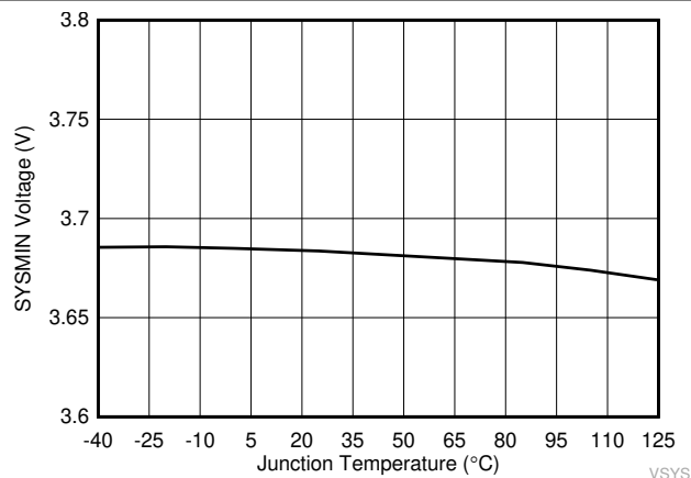
Figure 7-7. SYSMIN Voltage vs Junction Temperature (VSYs set at 3.5 V)
