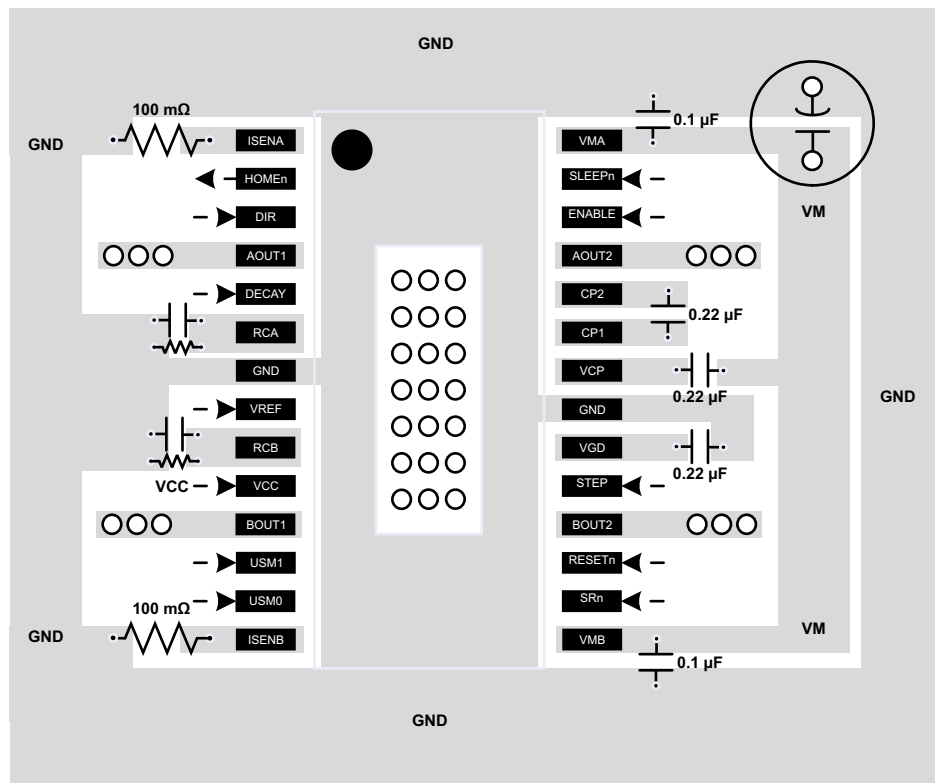
Figure 12. DRV8843 Layout Example
