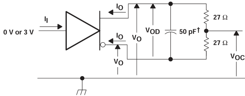
Figure 6-1. Driver Test Circuit, v_{OD} And v_{OC} Without Common-Mode Loading
