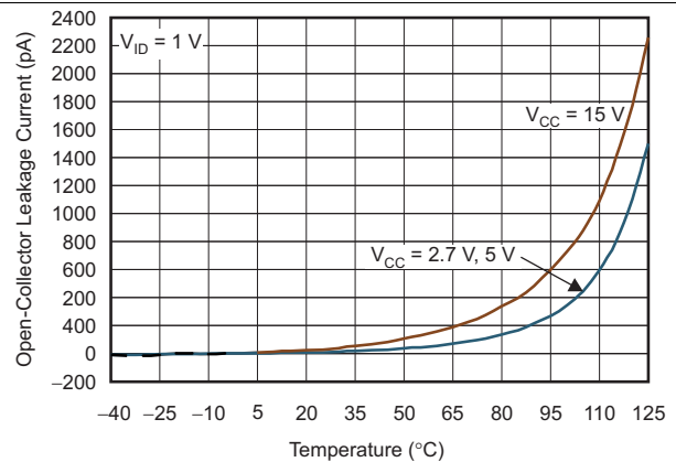
Figure 2. Open-Collector Leakage Current vs Free-Air Temperature
