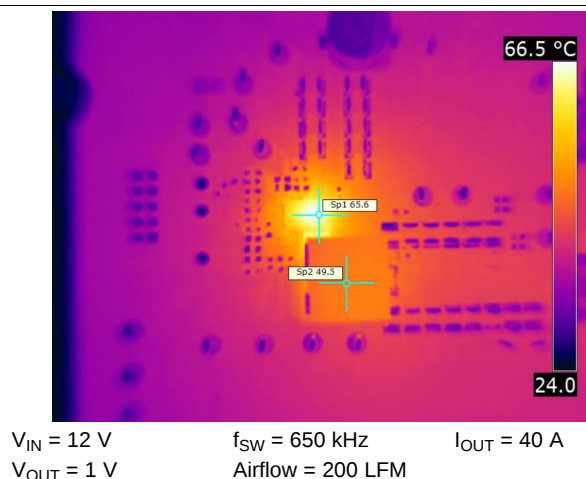
Figure 6. Thermal Image
