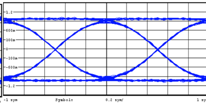
1.2 kbps, 2-FSK, DEV = 4 kHz Figure 4-8. Eye Diagram
