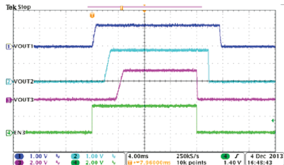
Figure 8-27. Automatic Power Sequencing, MODE = EN1 = EN2 = HIGH
