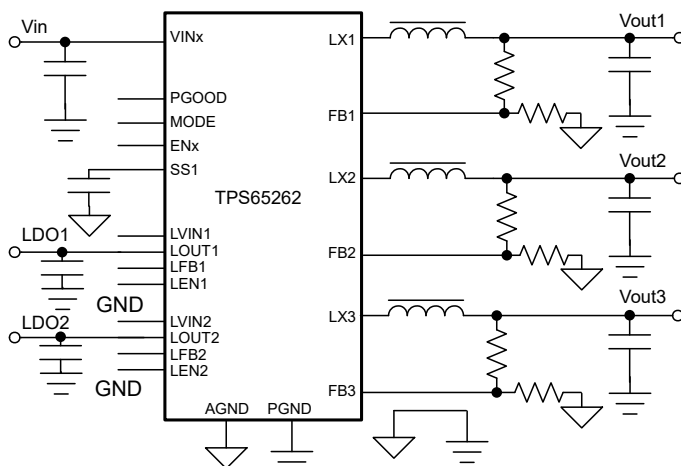
Application Schematic
