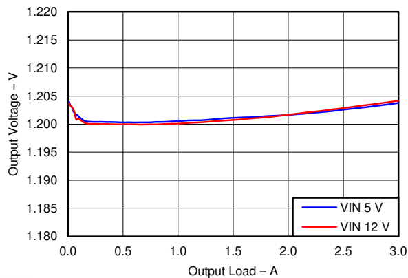
Figure 6-3. Buck1, Load Regulation
