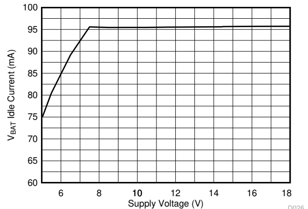
Figure 7-16. VBAT Idle Current vs Voltage
