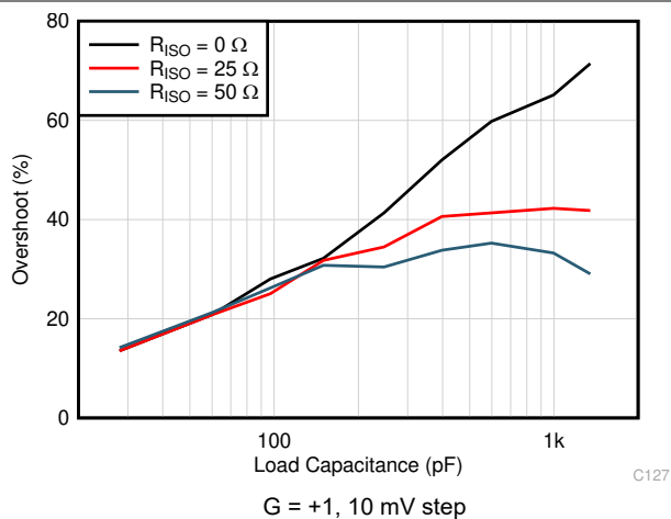
Figure 5-20. Small-Signal Overshoot vs Capacitive Load
