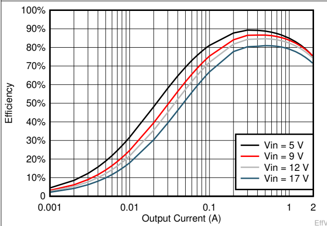
Figure 7-9. V_{OUT} = 0.95 V Efficiency, L = 2.2 \mu H
