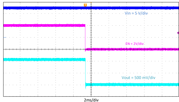
Figure 9-13. Shutdown Relative to EN
