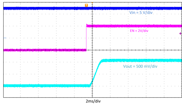
Figure 9-11. Start-Up Relative to EN
