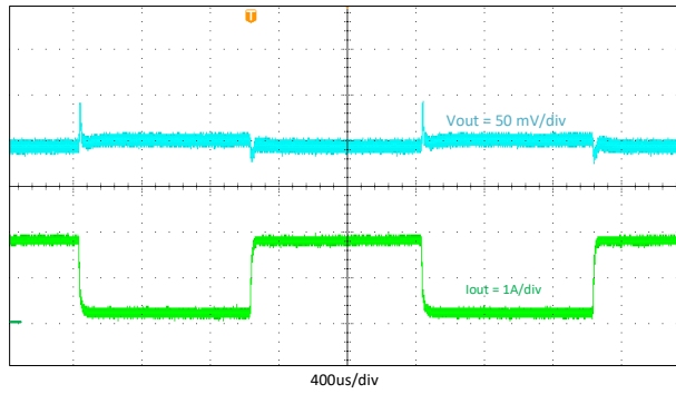
Figure 9-8. Transient Response, 0.2 to 1.8 A
