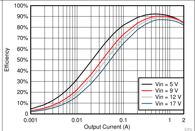
Figure 7-12. V_{OUT} = 1.8 V Efficiency, L = 2.2 \mu H
