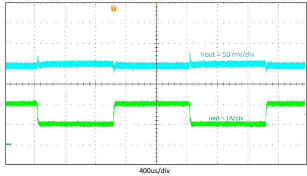
Figure 9-9. Transient Response, 1 to 2 A
