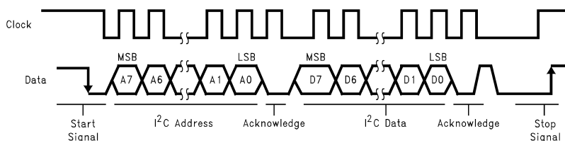
Figure 53. I 2 C Bus Format
