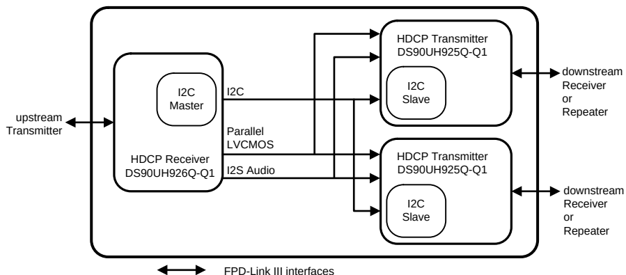
Figure 21. HDCP 1:2 Repeater Configuration
