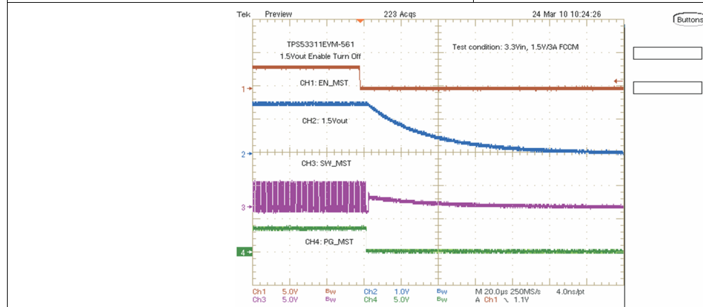
Figure 22. 1.5-V Turnoff Waveform
