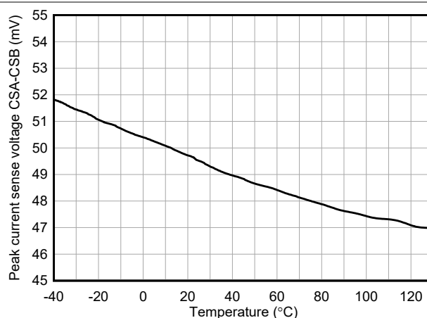
Figure 6-8. Current Limit Threshold Voltage versus Temperature
