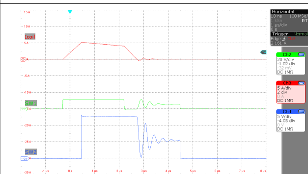
Figure 9-7. Inductor current buck-boost operation (MODE = 0\text{ V} , V_o = 12\text{ V} , I_o = 10\text{ mA} , V_{(VIN)} = 12\text{ V} )
