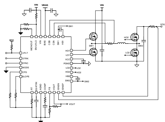
Simplified Schematic
