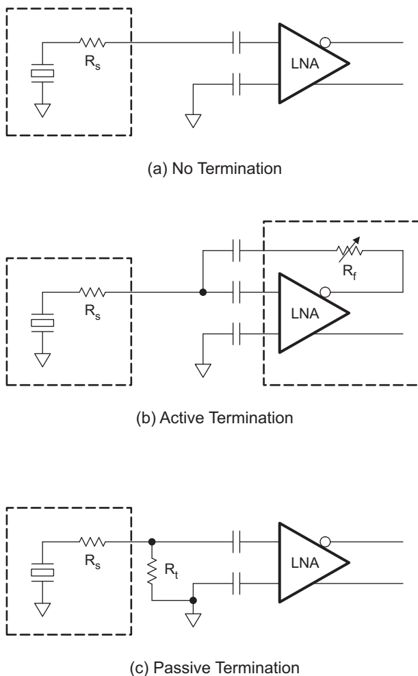
Figure 82. Termination Configurations
