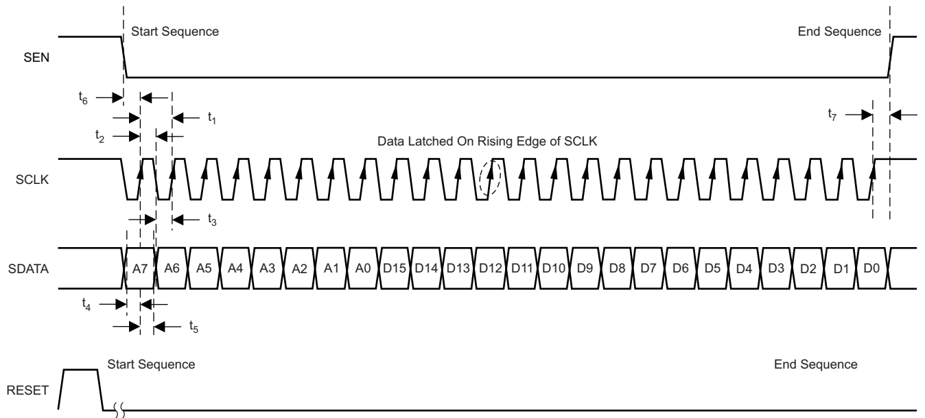
Figure 77. SPI Timing
