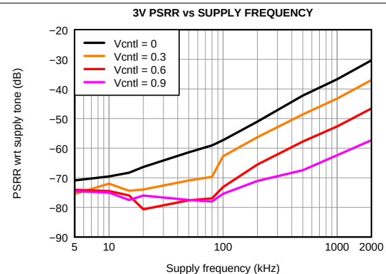
Figure 47. AVDD Power Supply Modulation Ratio
