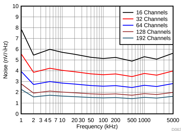
Figure 85. Allowed Noise on the VCNTL Signal Across Frequency and Different Channels
