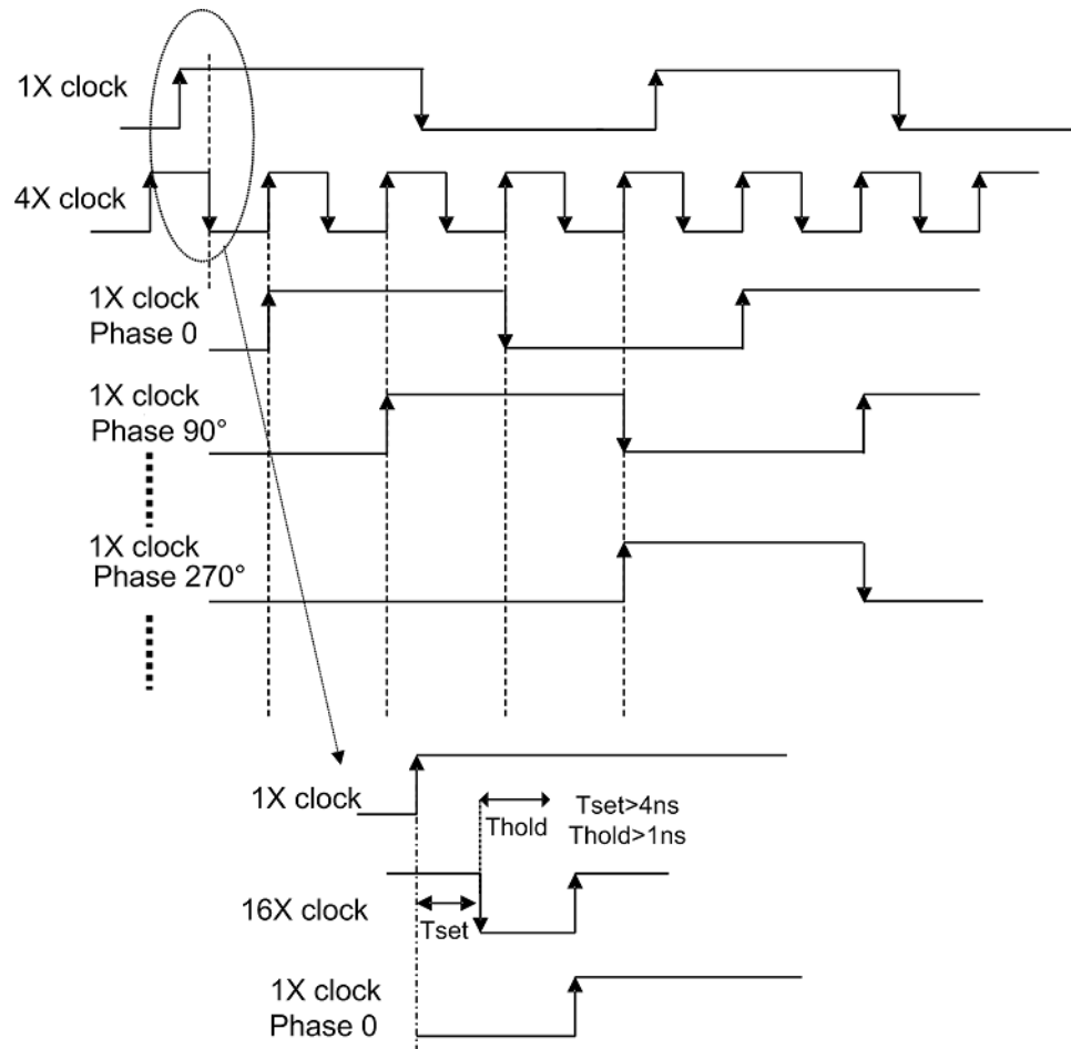
Figure 69. 8 \times f_{cw} and 4 \times f_{cw} Timing Diagram
