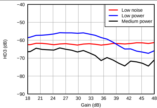
Figure 44. HD3 vs Gain
