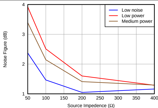
Figure 36. Noise Figure vs Power Modes Without Termination
