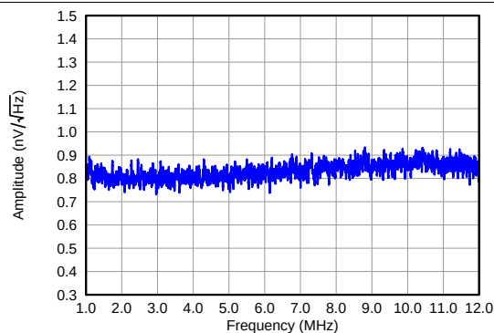
Figure 27. IRN and Low-Noise Mode
