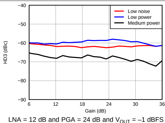
Figure 40. HD3 vs Gain
