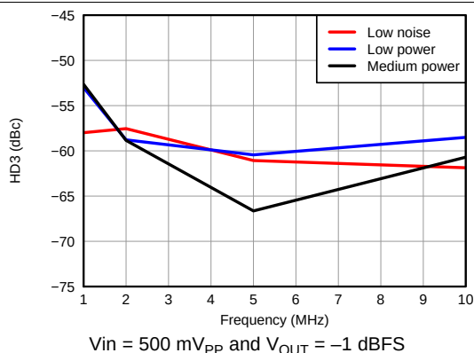
Figure 38. HD3 vs Frequency
