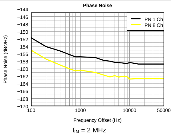
Figure 16. CW Phase Noise, 1 Channel vs 8 Channel
