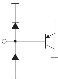
Figure 72. Equivalent Circuits of V_{\text{CNTLP/M}}
