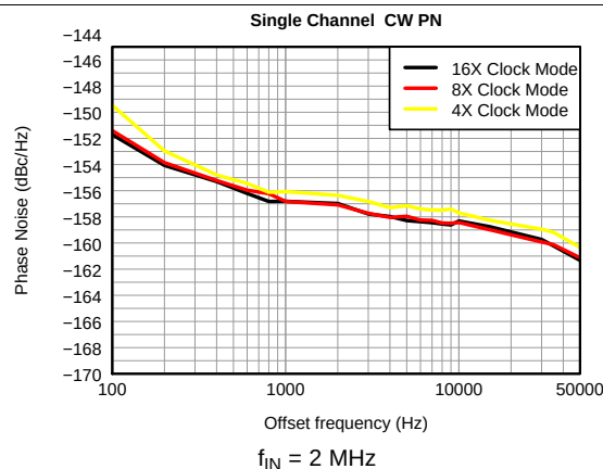
Figure 15. CW Phase Noise
