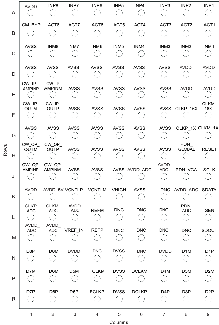
Pin Functions
