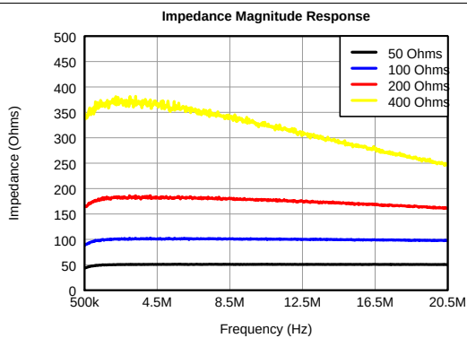
Figure 8. Input Impedance Without Active Termination (Magnitude)
