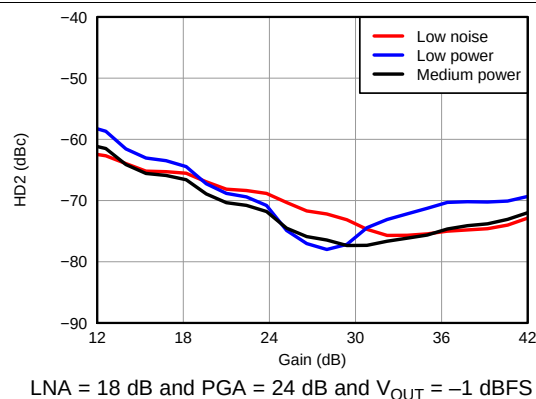
Figure 41. HD2 vs Gain
