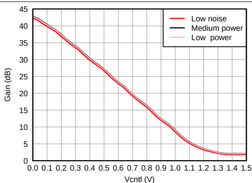
Figure 2. Gain vs VCNTL
