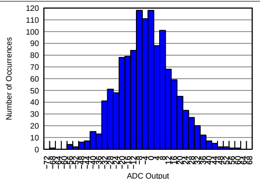
Figure 5. Gain Matching Histogram
