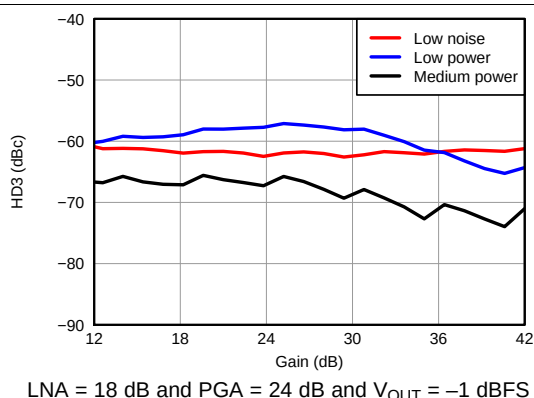
Figure 42. HD3 vs Gain
