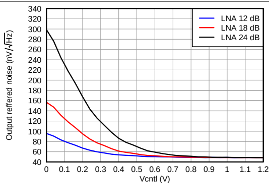
Figure 26. ORN and Low-Power Mode
