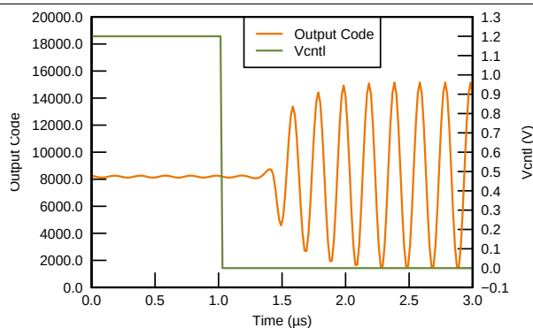
Figure 51. VCNTL Response Time
