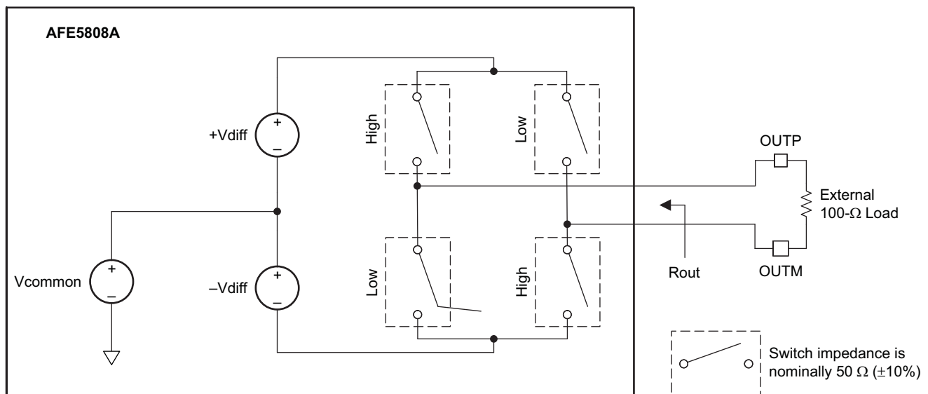
Figure 75. Equivalent Circuits of LVDS Outputs
