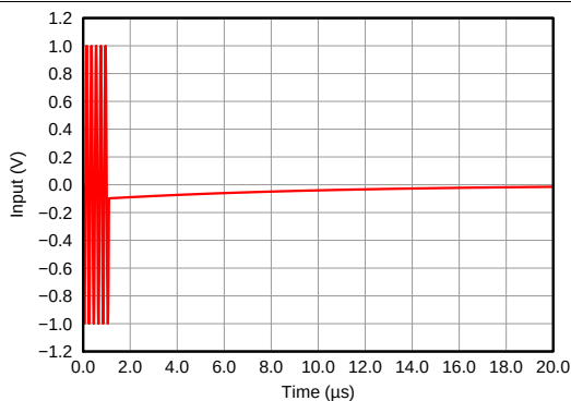
Figure 52. VCNTL Response Time
