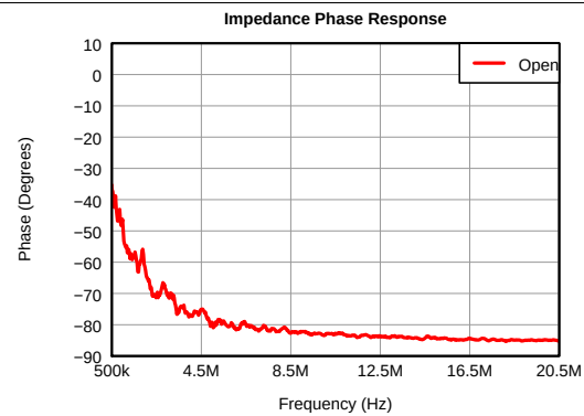
Figure 9. Input Impedance Without Active Termination (Phase)
