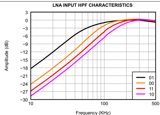
Figure 13. LNA High-Pass Filter Response vs Reg59 [3:2]
