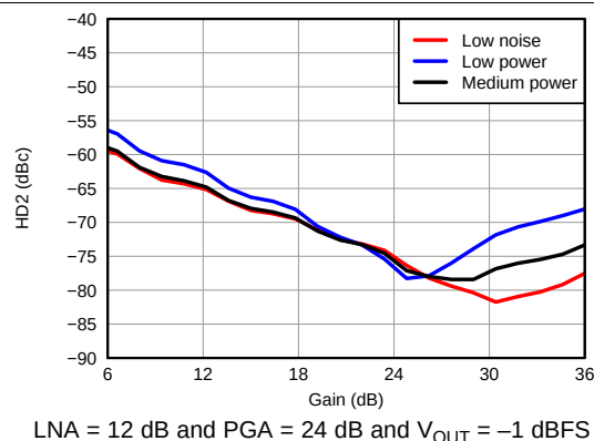
Figure 39. HD2 vs Gain
