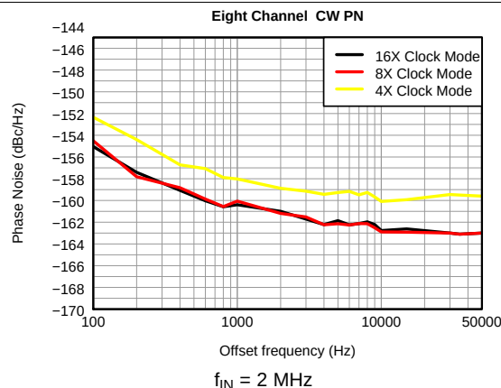
Figure 17. CW Phase Noise vs Clock Modes
