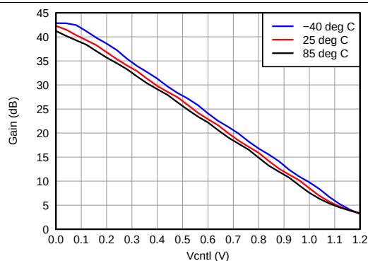
Figure 3. Gain Variation vs Temperature
