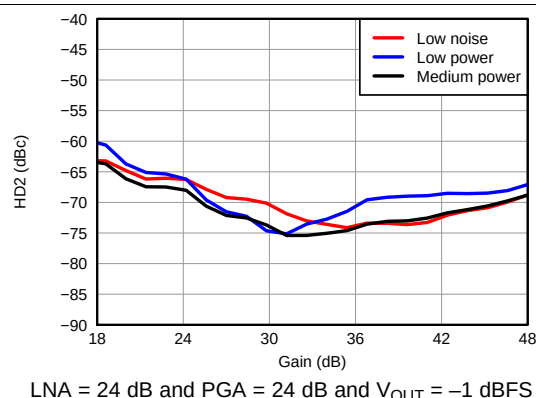
Figure 43. HD2 vs Gain
