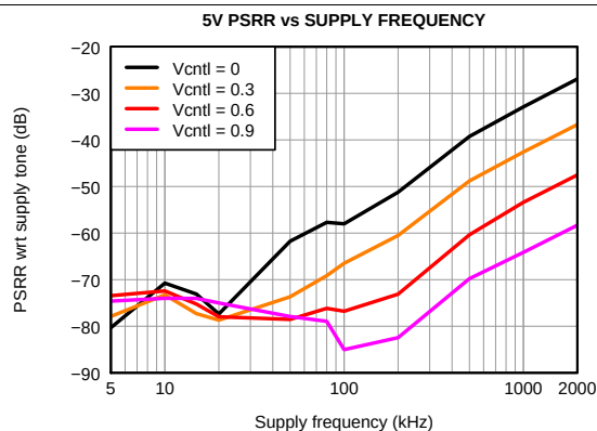
Figure 50. AVDD_5 V Power Supply Rejection Ratio
