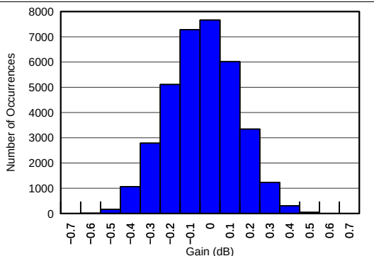
Figure 4. Gain Matching Histogram
