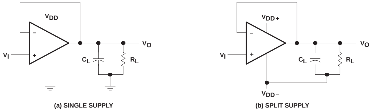
Figure 33. Unity-Gain Amplifier
