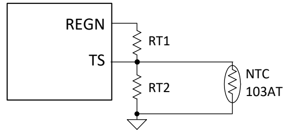
Figure 9-6. TS Pin Resistor Network
