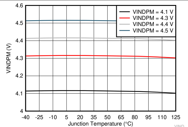
Figure 8-6. VINDPM vs Junction Temperature
