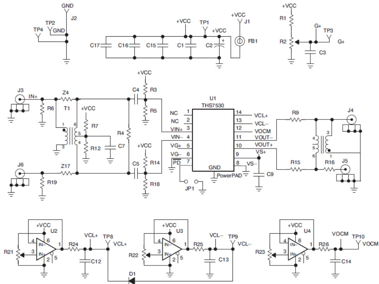
Figure 11-2. EVM Schematic
