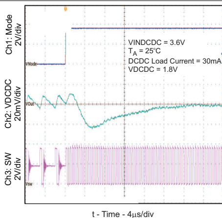
Figure 13. PFM to PWM Transition (DC-DC)
