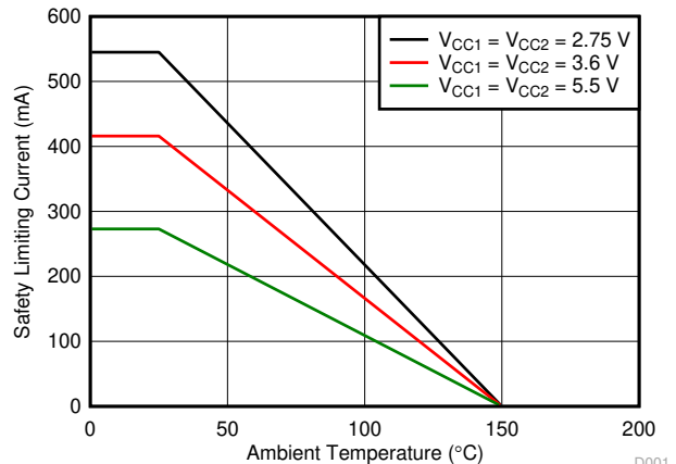
Figure 5-2. Thermal Derating Curve for Safety Limiting Current for DW-16 Package
