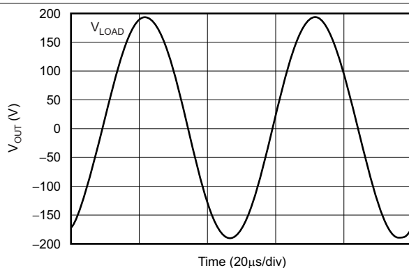
Figure 82. 390 V PP Across 7.5-kΩ Load 20 kHz, Uses Six OPA454s, 100-V Supplies
