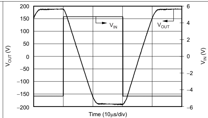
Figure 83. 7.5-kΩ Load, G = +20, Six OPA454s, 100-V Supplies
