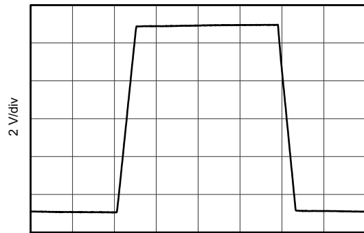
Time (50 \mu s/div) G = +1 , R_L = 10 k \Omega , C_L = 10 pF
